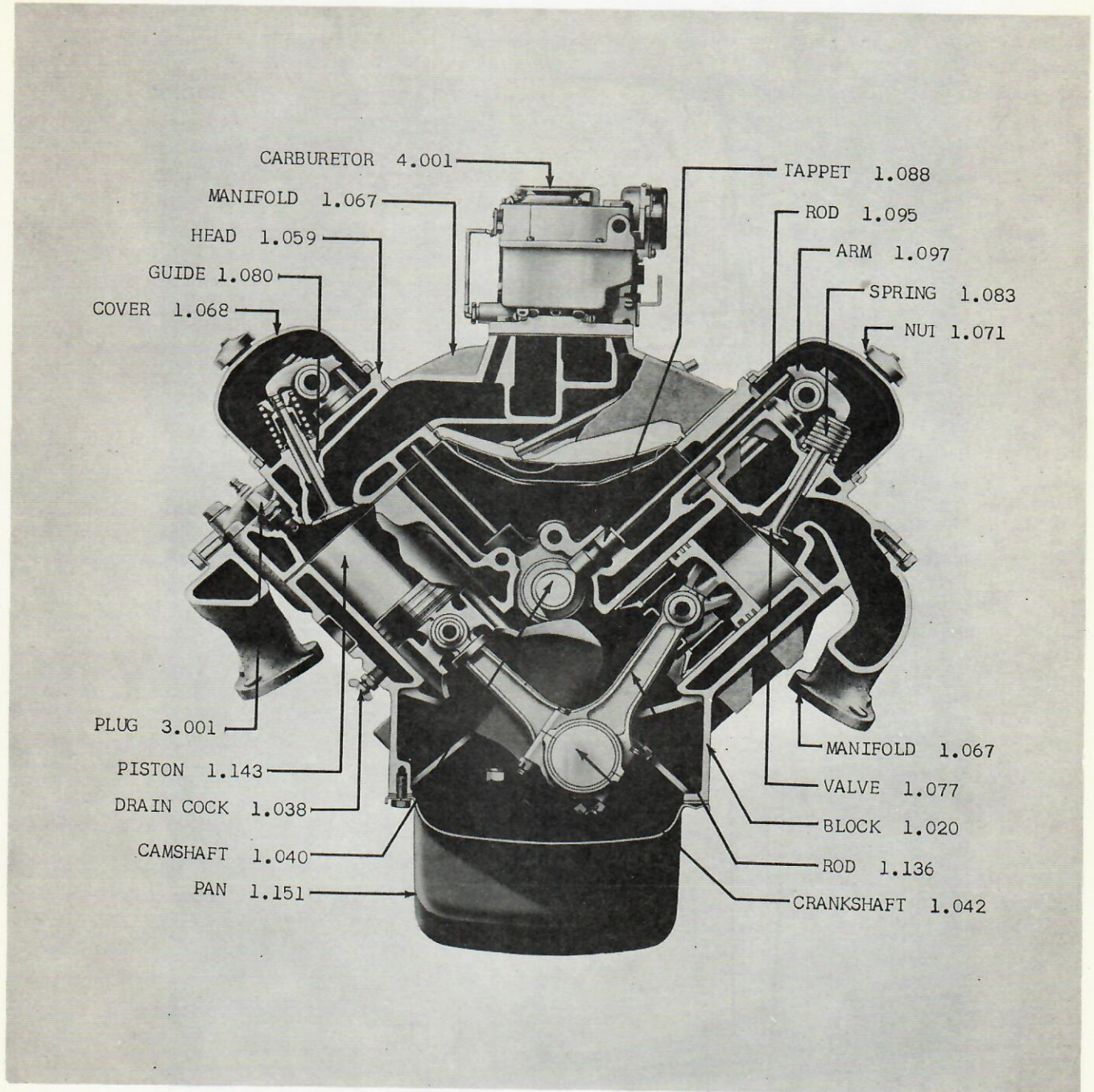
GROUP 0 - FIG. 13 ENGINE ASSEMBLY V-8 20-80
