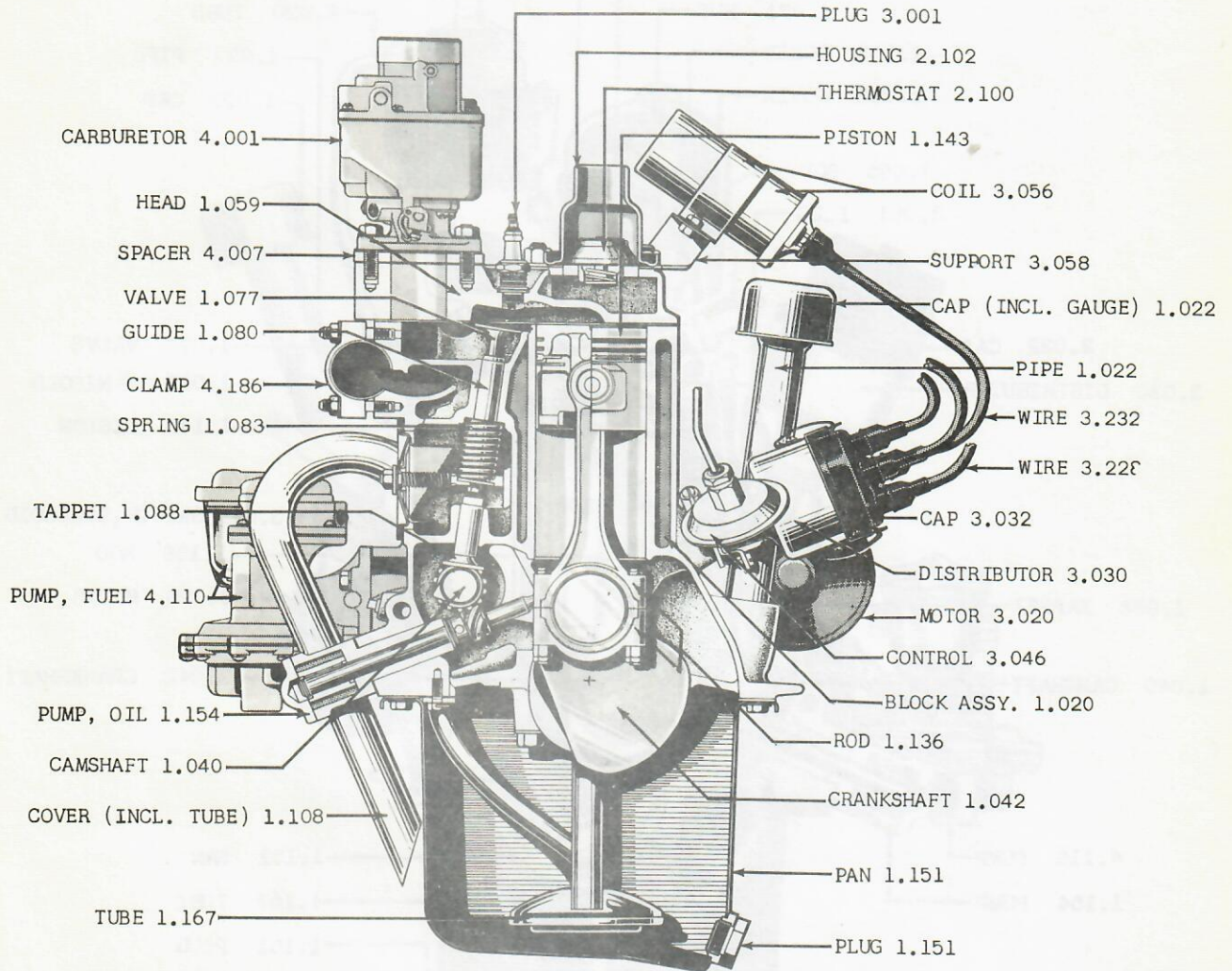
GROUP 0 - FIG. 11 - ENGINE ASSEMBLY "L" HEAD 6 01
